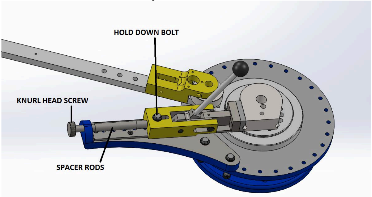
Figure 3: Clamping pressure adjustment
